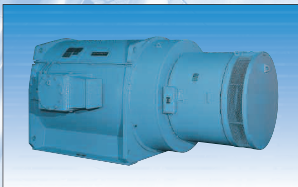
Converter-fed drive for screw-type kneader, Exd IIC T4, 1,500 kW, 900 V, 600 - 1,600 rpm; independent cooling
