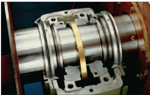
Sleeve bearing with ring oiler
