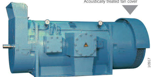
Motor with air outlet absorber and acoustically treated frame mantle
