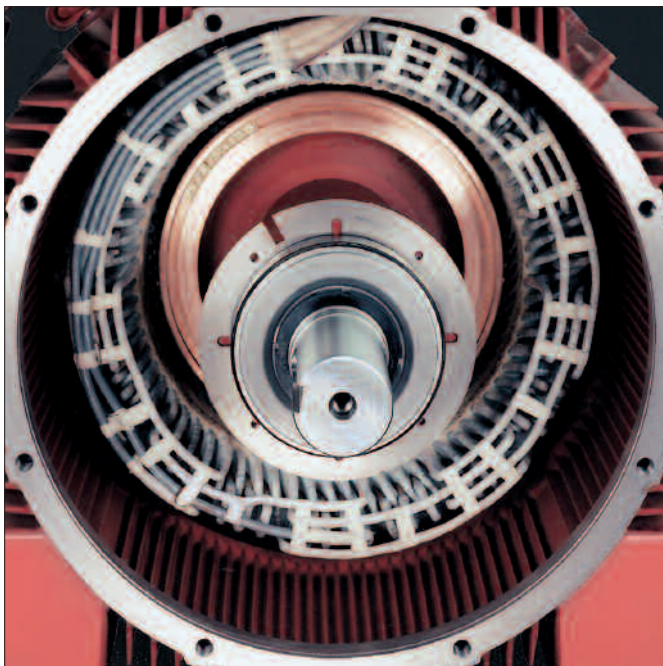
Connecting side of endwinding
