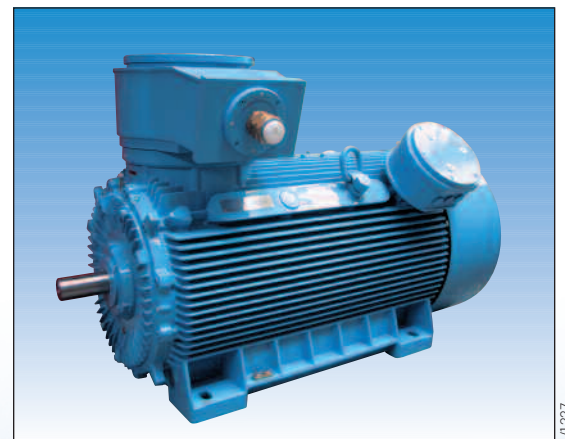
Drive for screw-type compressor, Exd IIC T4, 315 kW, 6 kV, 2-pole
